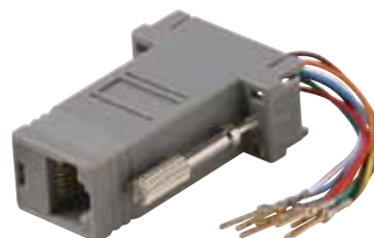
504-207 DE9 Male to 6x6 Modular Adapter 504-209 DE9 Male to 8x8 Modular Adapter
