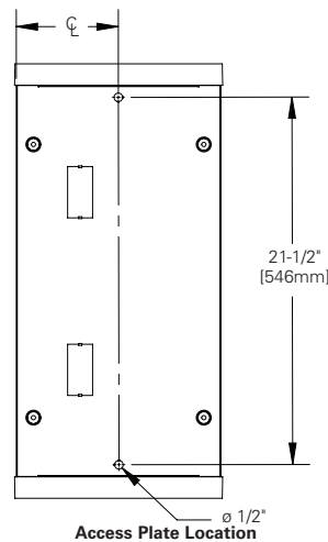
Access Plate Location
