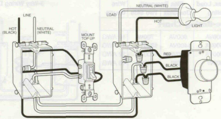
Rotary Dimmer 3-Way Wiring Diagram
