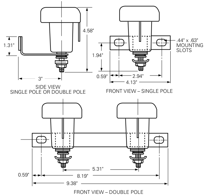
Figure 7. Type S4 secondary arresters dimensional information.
