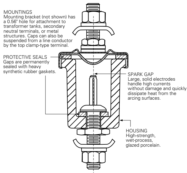
Figure 9. Cutaway illustration of protective gap.
