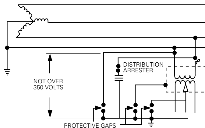
Figure 10. Typical application of protective gaps.
