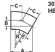
30° Horizontal Bend
