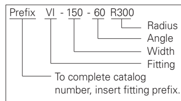
60° (VI) Mitered
