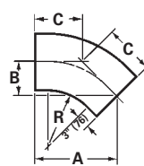
45° HB
