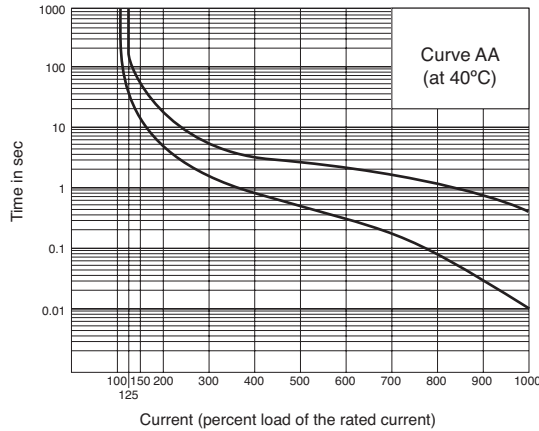
AC (50/60 Hz) Time Delay Curves
