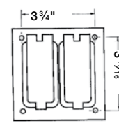
Typical FS mount hole pattern
