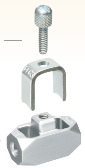
FLG3 Exploded view
