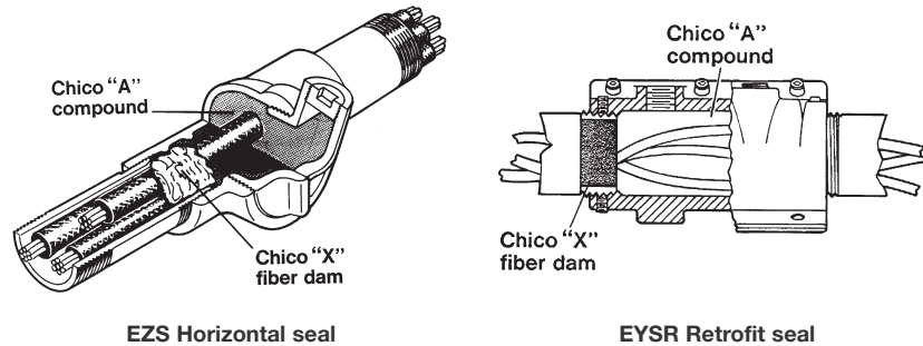
EZS Horizontal seal
