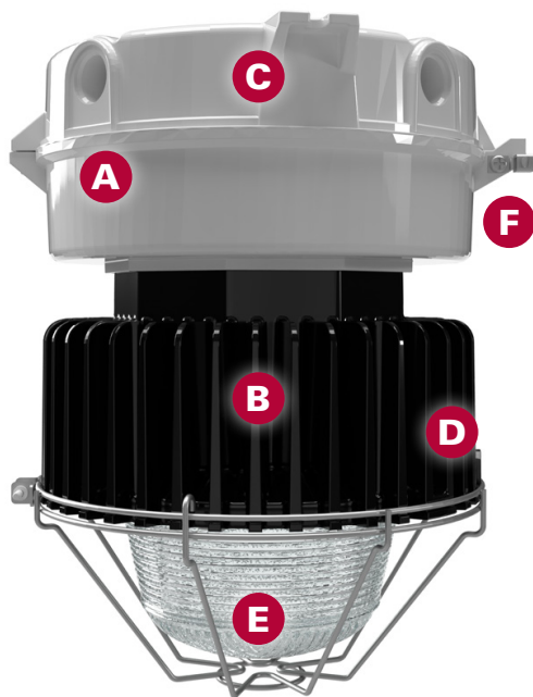
VMVL-3 – VMVL-13 shown w optional uplight refractor lens and wire guard
