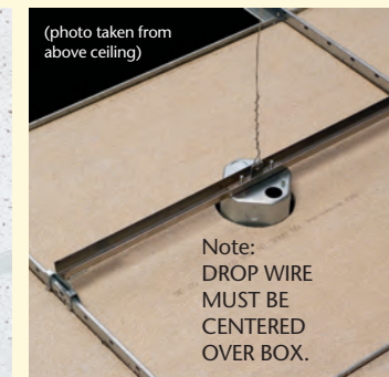
2 Place box over hole. Note: DROP WIRE MUST BE CENTERED OVER BOX.
