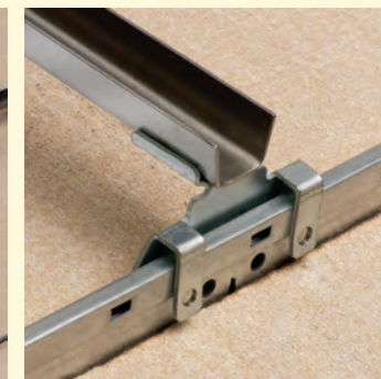
3 Snap ends of support bar over the ceiling grid (tees).
