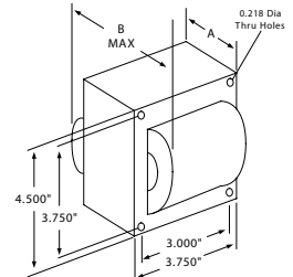
REFERENCE DRAWING 2
