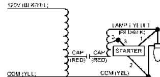
Wiring Diagram 13
