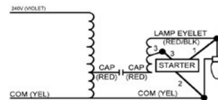
Wiring Diagram 14
