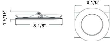
RT609WH/FR/P Frosted Glass Lens with White Plastic Ring Uses 11-27W GU24 Lamps Order Code: 79155
