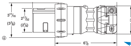
Plug
