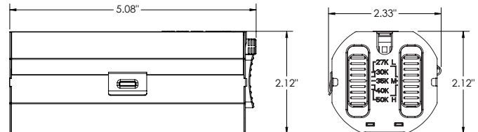
2 1/2" CEILING CUTOUT
